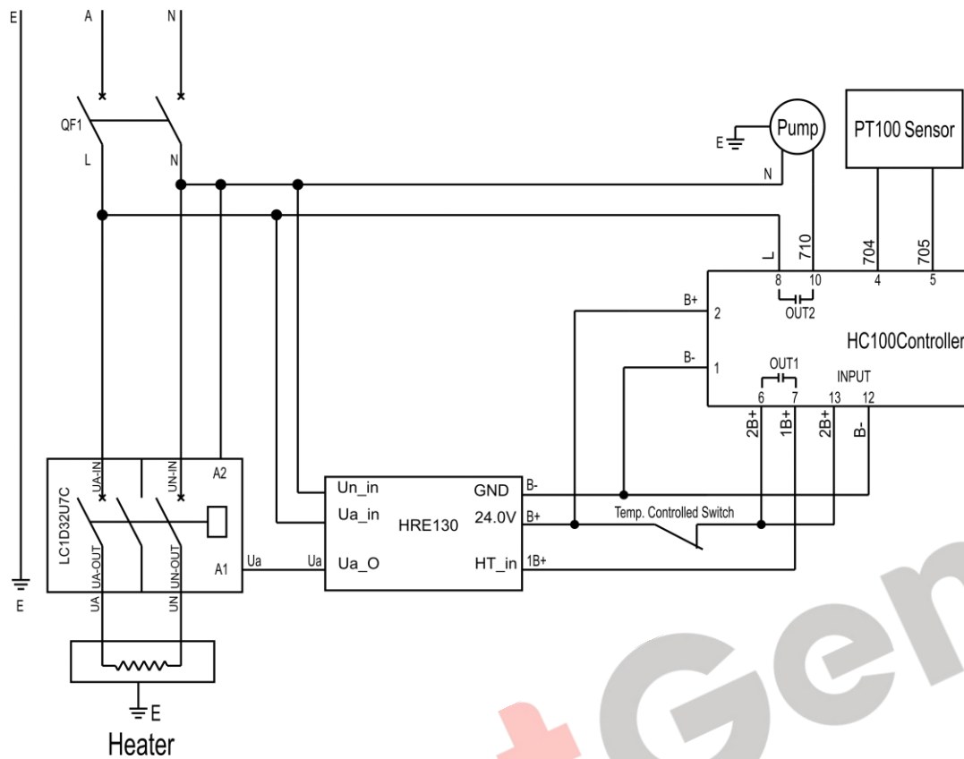
Fig.5 - HWP40 Diagram
