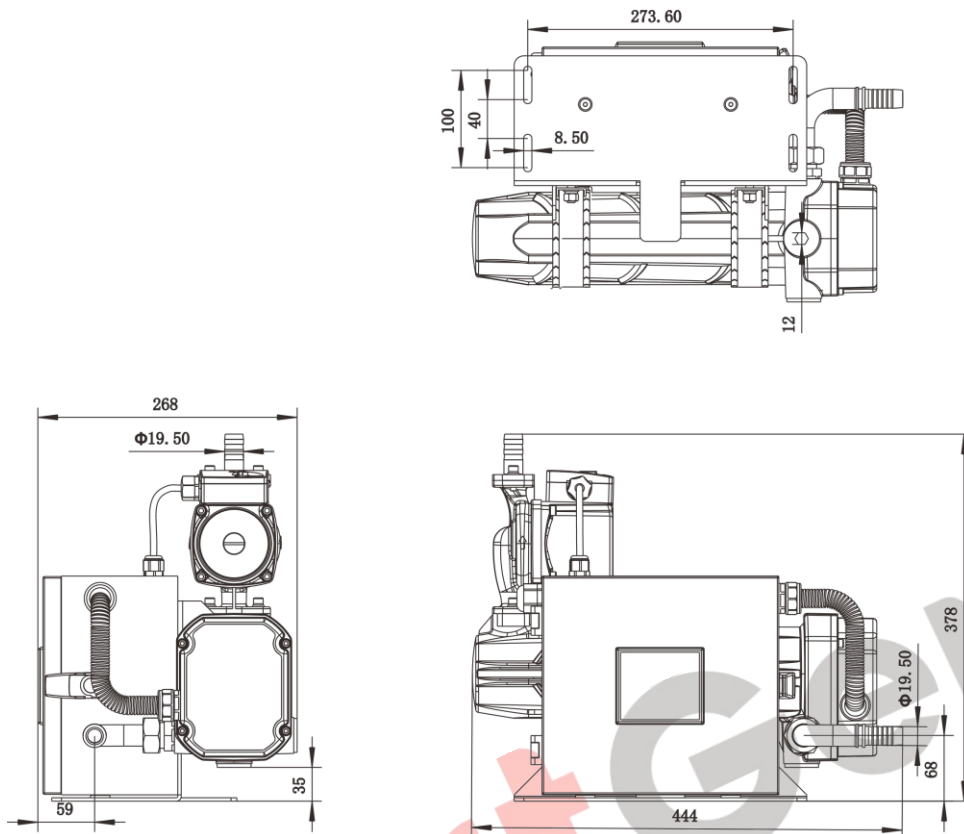
Fig.7 – Overall Dimensions
